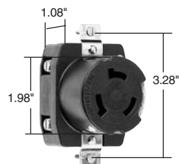
Corrosion-Resistant Receptacle
